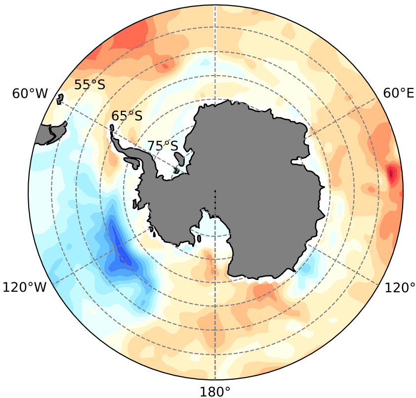
C (CESM2-NUDGE)
