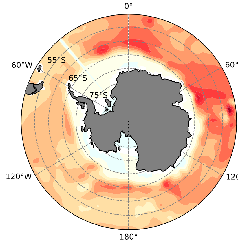
B CESM2-FORECAST-2024
