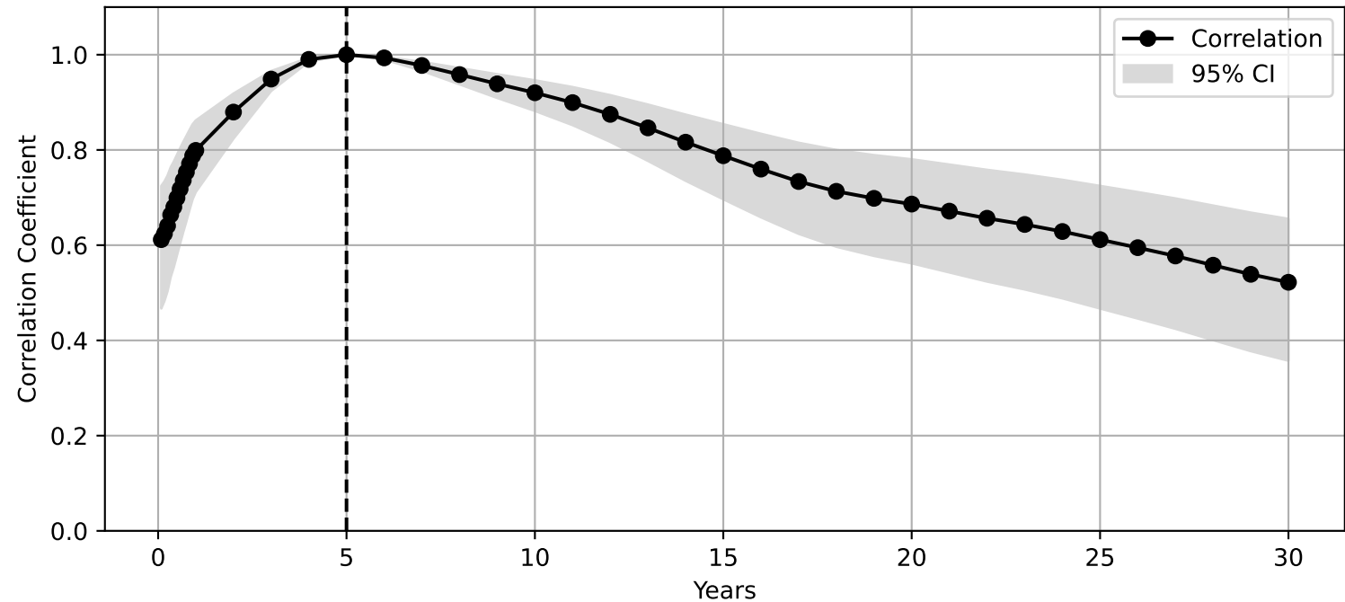
Correlation of SO-EPT 5year with SO-EPT xyear
