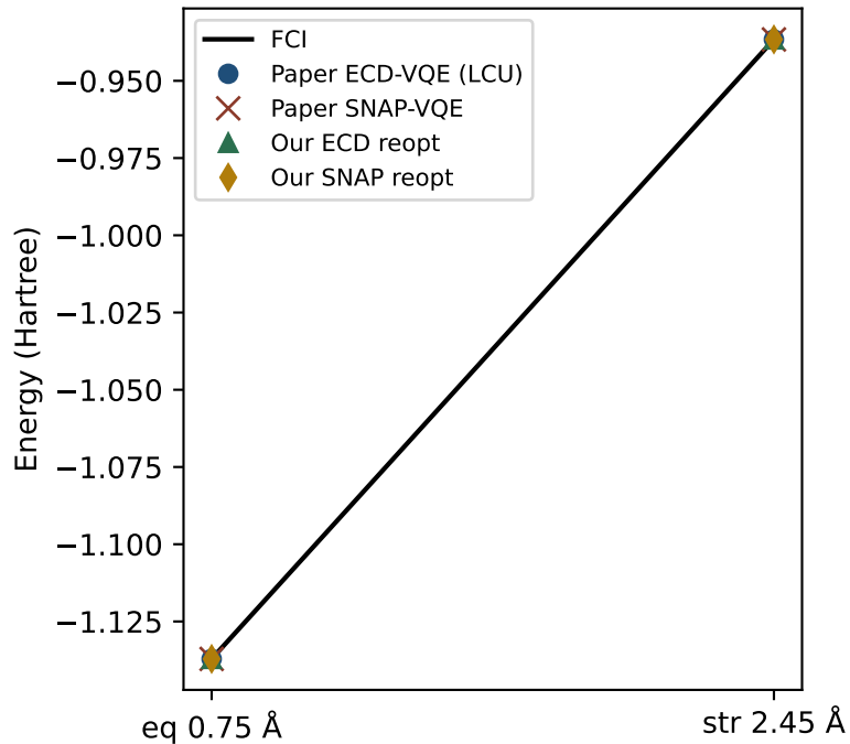
H2 STO-3G, two bond lengths
