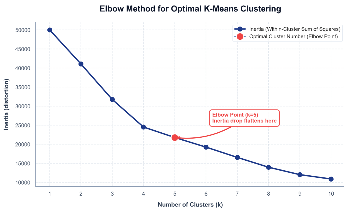
Figure 3.2: Elbow method showing inertia drop rates across clusters.
