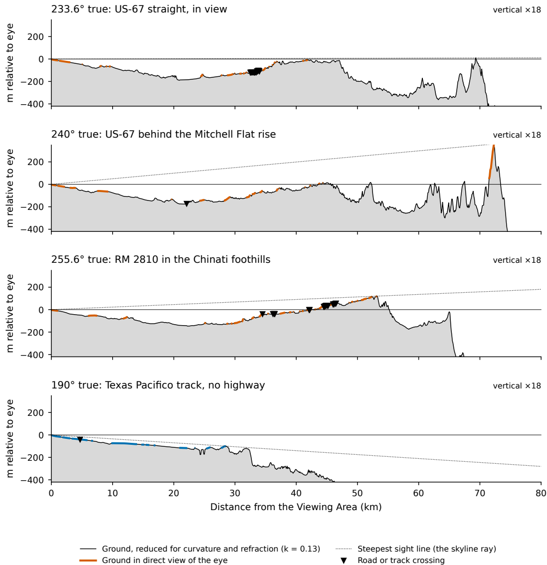
Figure S1: Terrain cross-sections from the platform along four bearings, reduced for curvature and refraction ( k = 0.13 ), exaggerated 18\times vertically. Colored: ground in direct view of the eye. Triangles: road or track crossings. Along 233.6^\circ the view skims the far slope that carries US-67; along 240^\circ a low rise hides the highway.
