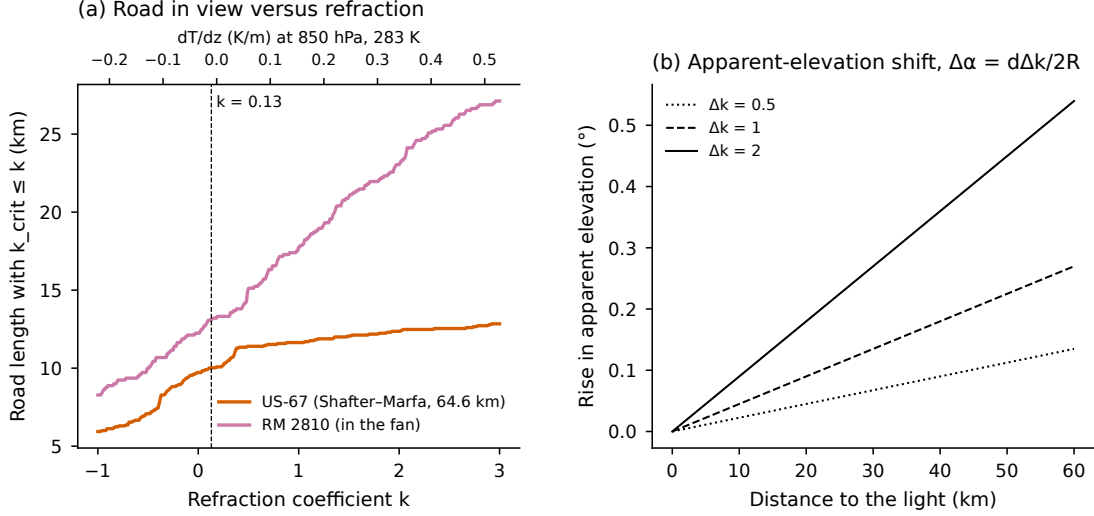
Figure S2: (a) Road in view (constant- k model) versus refraction coefficient; the top axis gives the equivalent temperature gradient from Eq. (4). (b) Rise in apparent elevation for a change \Delta k , d\Delta k/2R .
