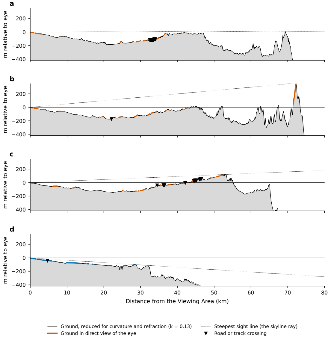
Figure S1: Terrain cross-sections from the platform, reduced for curvature and refraction ( k = 0.13 ), exaggerated 18 \times vertically, along (a) 233.6° true, where the view skims the far slope that carries a straight stretch of US-67 in view; (b) 240°, where a low rise on Mitchell Flat hides the highway; (c) 255.6°, across RM 2810 in the Chinati foothills; (d) 190°, along the Texas Pacifico railroad, with no highway. Colored: ground in direct view of the eye. Triangles: road or track crossings.
