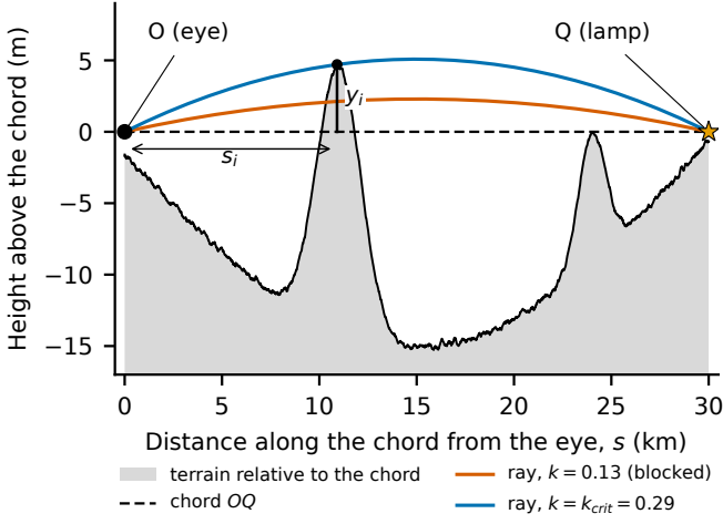
FIG. 2. Line-of-sight geometry in the frame of the straight chord OQ (illustrative profile, 30 km). The terrain is plotted as its height y above the chord, which includes Earth’s curvature. A refracted ray with coefficient k lies above the chord by ks(D-s)/2R . Here the ridge at s_i , which rises y_i above the chord, blocks the standard ray ( k = 0.13 ); the lamp becomes visible for k \geq k_{\text{crit}} = 0.29 .
