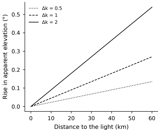
(b) Apparent-elevation shift, \Delta\alpha = d\Delta k/2R
