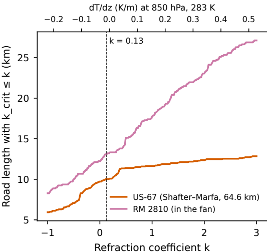
(a) Road in view versus refraction
