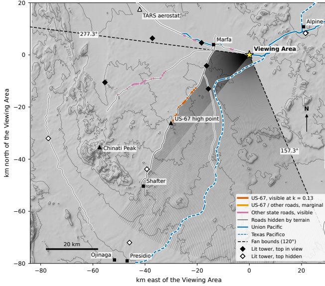
FIG. 1. The view from the Marfa lights viewing area (star) toward the southwest. Roads are colored where a headlamp is in direct view of the platform (Sec. VI). Diamonds are lit communication towers. The shaded fan shows rays every 0.5^\circ between 157.3^\circ and 277.3^\circ true.
