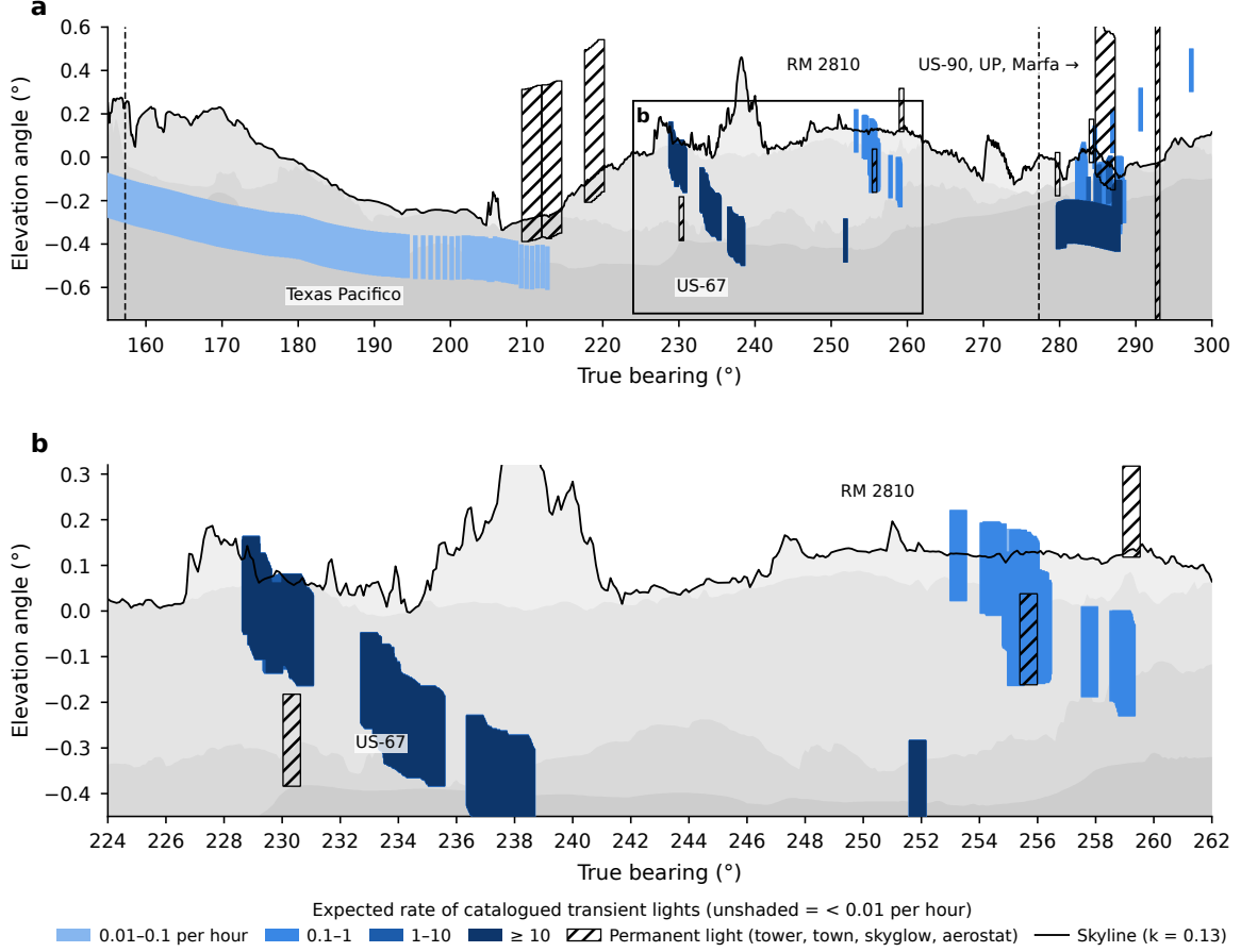
Figure S3: Expected rate of catalogued transient lights (per hour) across the view on a standard night ( k = 0.13 , V = 111 \text{ km} , pointing error \pm 0.3^\circ \times \pm 0.1^\circ ), with fixed lights hatched. (a) 155^\circ – 300^\circ , vertical scale exaggerated 29\times ; the box is the region of (b). (b) The US-67 and RM 2810 sector, 224^\circ – 262^\circ , exaggerated 16\times . Northbound US-67 traffic reaches about 23 lights per hour and RM 2810 at most 0.5; the Texas Pacific track carries at most 0.08 trains per hour.
