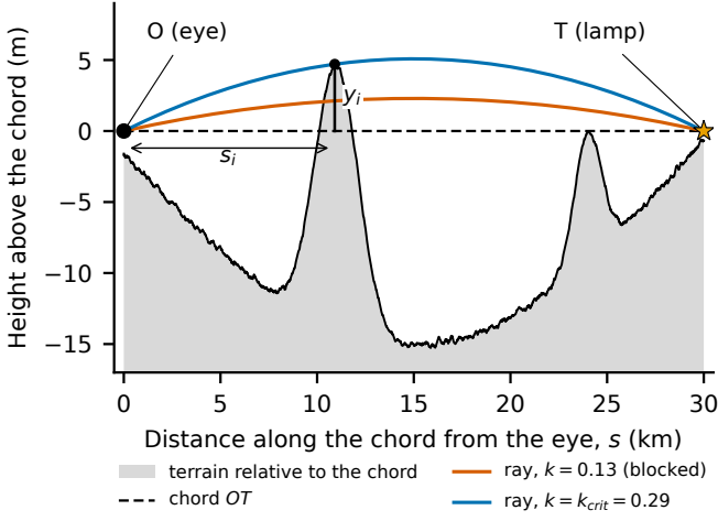
FIG. 2. Line-of-sight geometry in the frame of the straight chord OT (illustrative profile, 30 km). The terrain is plotted as its height y above the chord, which includes Earth’s curvature. A refracted ray with coefficient k lies above the chord by ks(D-s)/2R . Here the ridge at s_i , which rises y_i above the chord, blocks the standard ray ( k = 0.13 ); the lamp becomes visible for k \geq k_{\text{crit}} = 0.29 .
