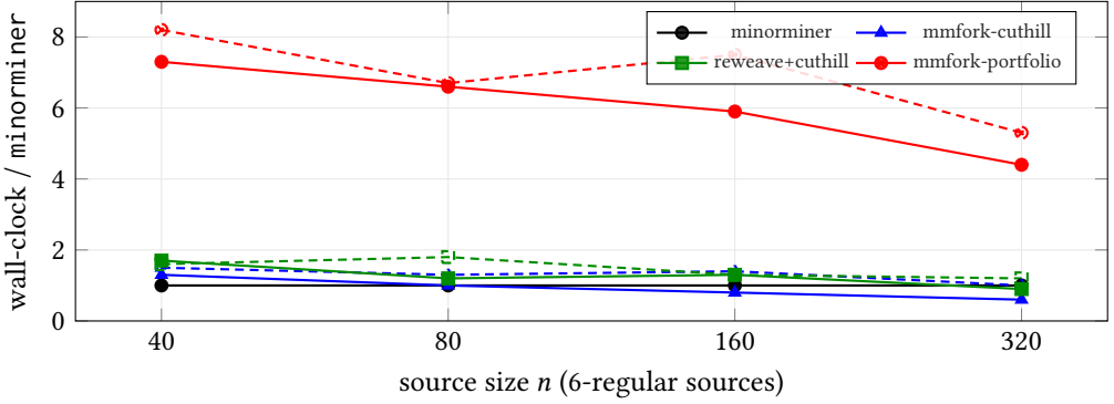
Fig. 6. Wall-clock relative to minorminer ( = 1 ) versus source size n (6-regular sources; solid = Advantage2 Z_{15} , dashed = Advantage P_{16} ; 5% faults). Every guided method’s multiplier shrinks with n : mmfork-cuthill and reweave-mmfork-cuthill fall below 1 (faster than stock minorminer) on the largest Z_{15} problems, and even the six-search portfolio’s premium nearly halves. The fixed cost of guidance amortizes against minorminer’s super-linearly-growing search.
