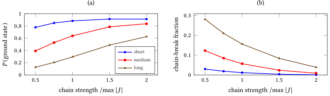
Fig. 9. The chain-strength sweep, by ACL tertile (short \leq 1.36 , medium, long \geq 1.78 ). (a) longer chains need a stronger ferromagnet and still cap at a lower P(\text{GS}) ; (b) at every chain strength the break fraction grows with chain length. Spending coupler budget to hold long chains rigid is budget taken from the logical problem—the cost that ACL measures.
