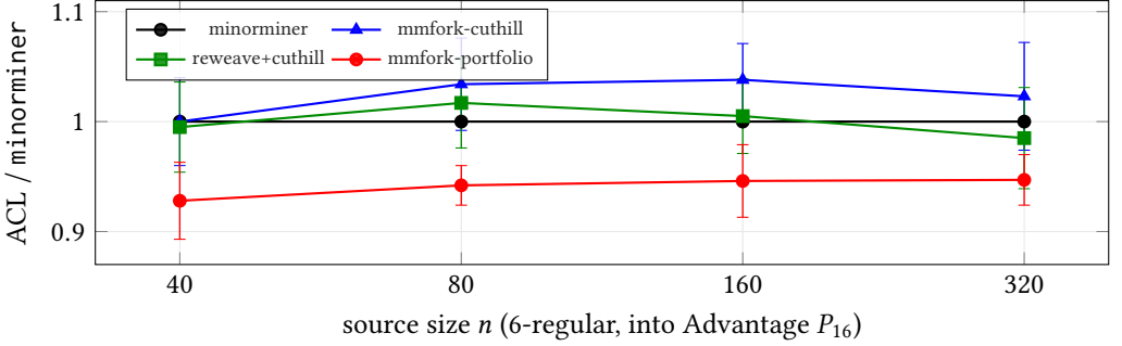
Fig. 7. ACL relative to minorminer ( = 1 ) versus n (6-regular into Advantage P_{16} ; mean over K=8 instances, 95% CI bars). mmfork-portfolio sits a consistent 5–7% below minorminer at every size (CI clears 1 throughout)—the advantage persists rather than widening; the single-order variants are within noise of minorminer on this sparse regime.
