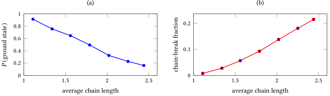
Fig. 8. Solution quality versus chain length across all 2,736 (problem, embedding) pairs (binned mean, reference chain strength). (a) the ground-state probability falls monotonically with ACL ( \rho = -0.63 , p \approx 10^{-296} ); (b) the chain-break fraction rises with ACL ( \rho = +0.80 )—the mechanism. Lower ACL is better on both axes.
