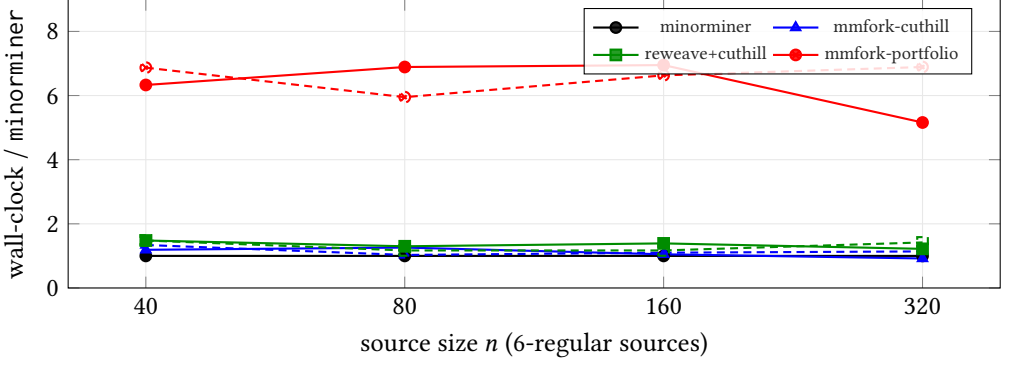
Fig. 6. Wall-clock relative to minorminer ( = 1 ) versus source size n (6-regular sources, mean over K=8 instances; solid = Advantage2 Z_{15} , dashed = Advantage P_{16} ; 5% faults). The guided methods’ multipliers stay bounded —flat-to-falling—rather than compounding with minorminer’s super-linearly-growing search: the single order mmfork-cuthill reaches parity ( 0.9\times ) on the largest Z_{15} problems, and the six-search portfolio’s \sim 6\times does not grow with n .
