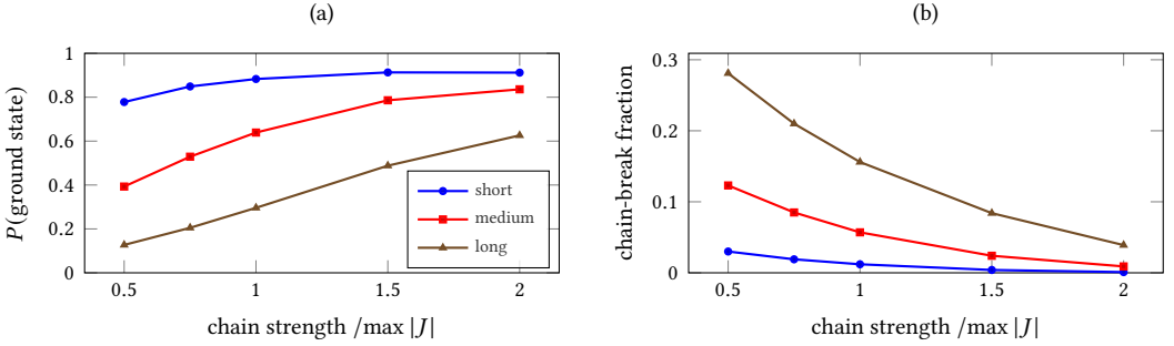
Fig. 9. The chain-strength sweep, by ACL tertile (short \leq 1.36 , medium, long \geq 1.78 ). (a) longer chains need a stronger ferromagnet and still cap at a lower P(\text{GS}) ; (b) at every chain strength the break fraction grows with chain length. Spending coupler budget to hold long chains rigid is budget taken from the logical problem—the cost that ACL measures.
