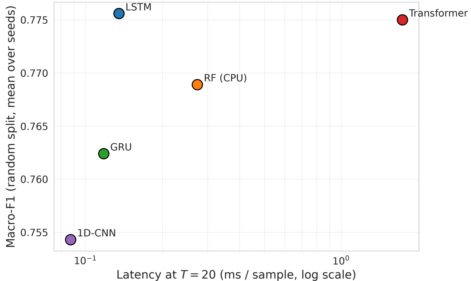
Cost vs accuracy at T = 20
