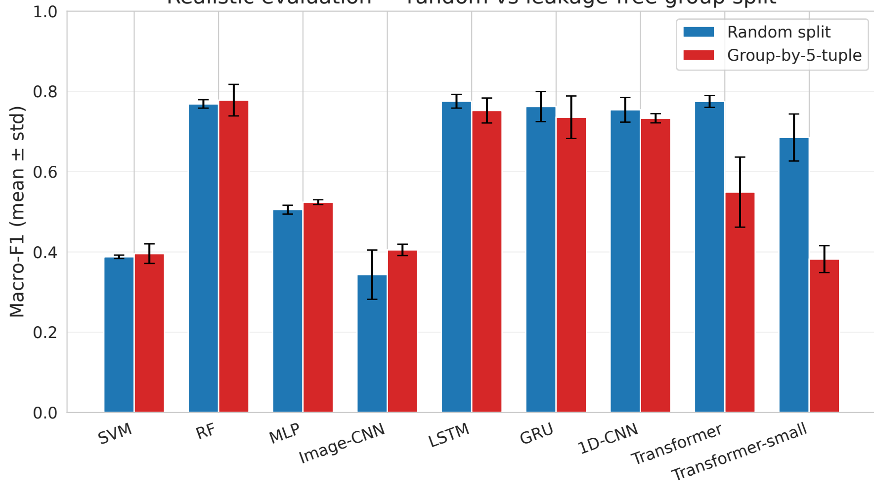
Realistic evaluation — random vs leakage-free group split
