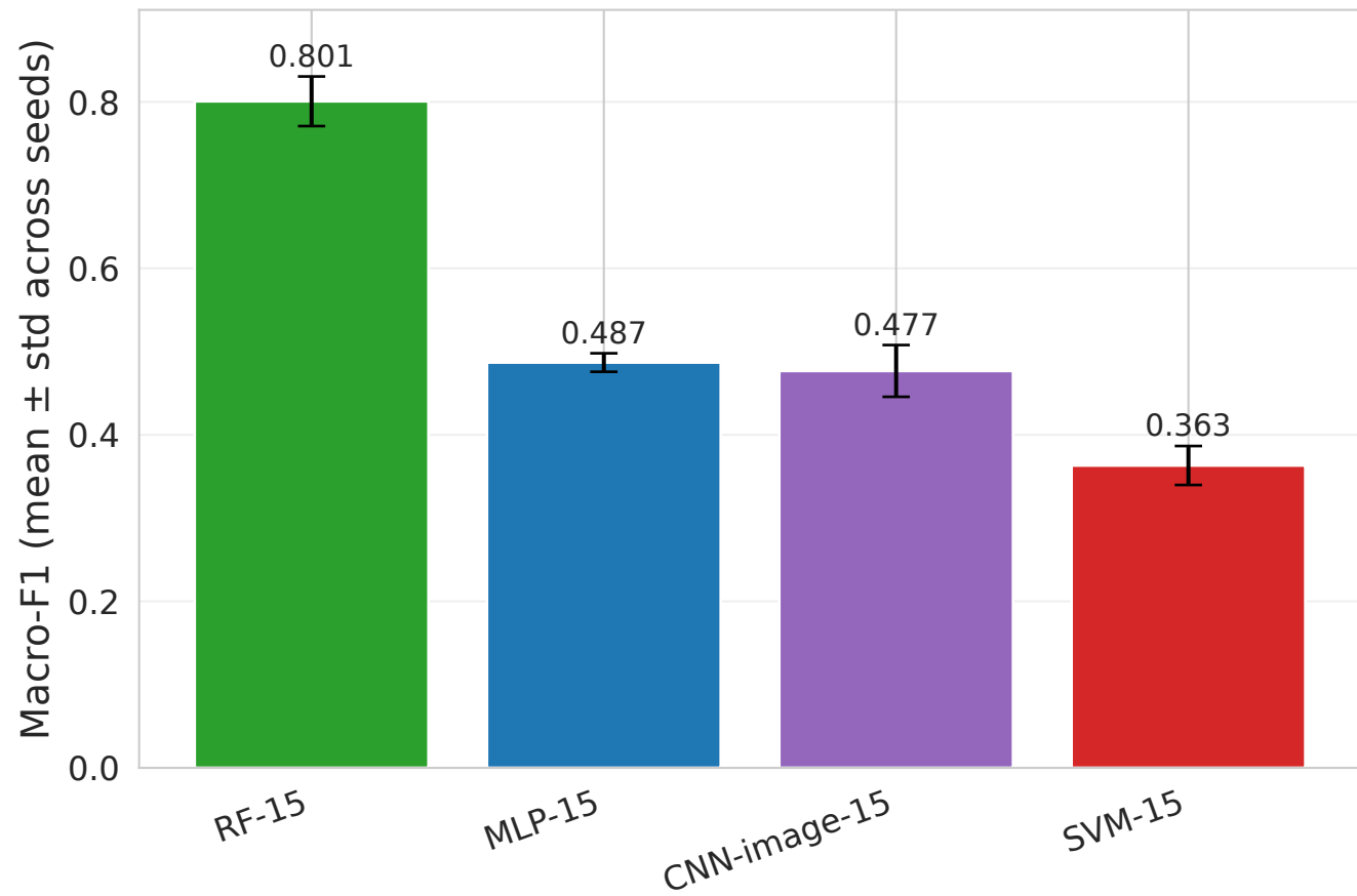
Static models on the full 15-class flow data
