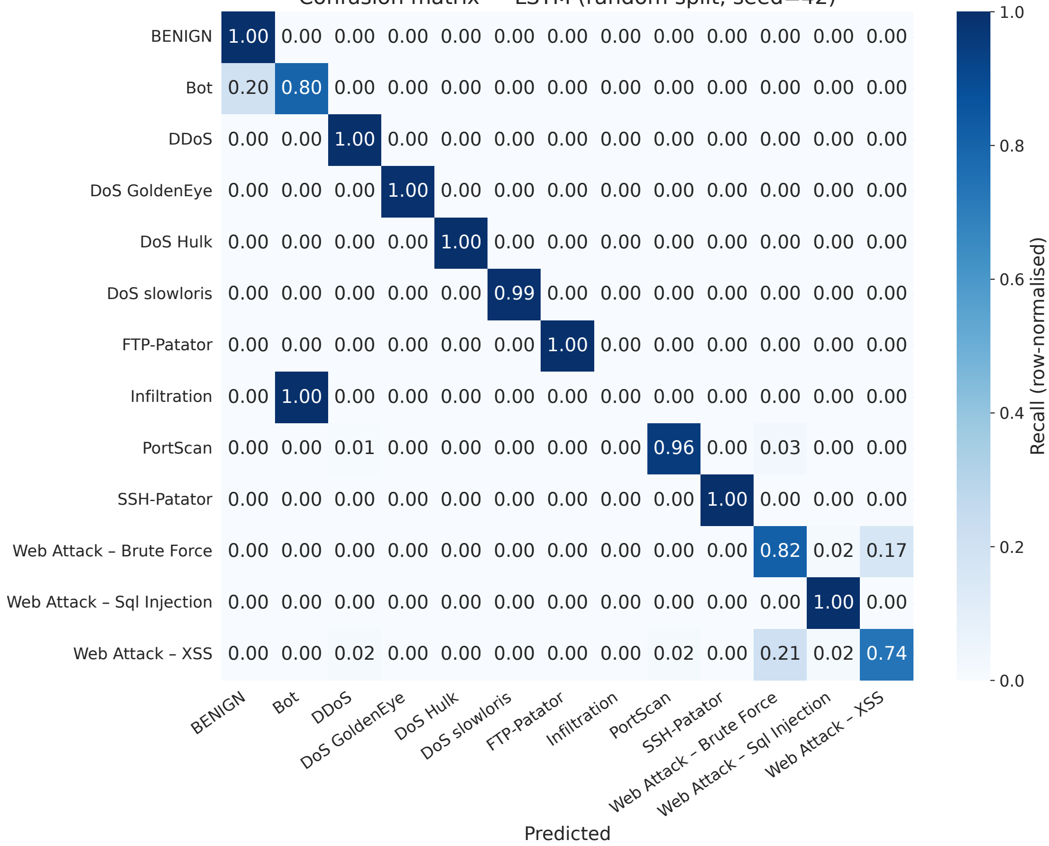
Confusion matrix — LSTM (random split, seed=42)
