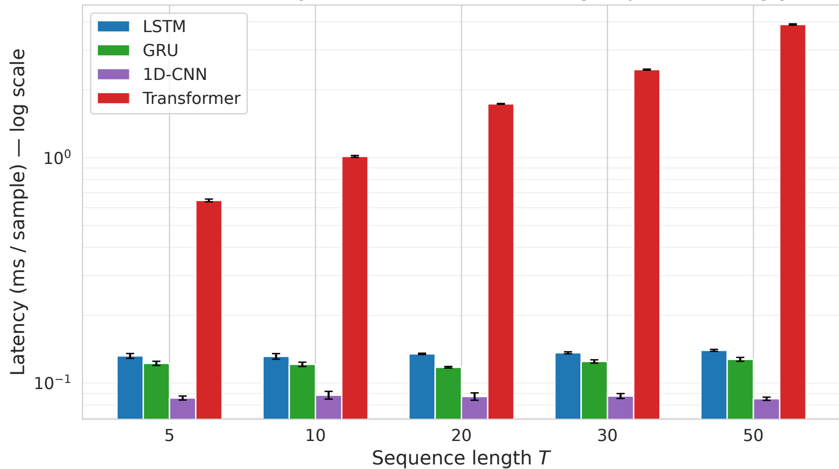
Inference latency vs T on NVIDIA A100 — grouped bars (log-y)
