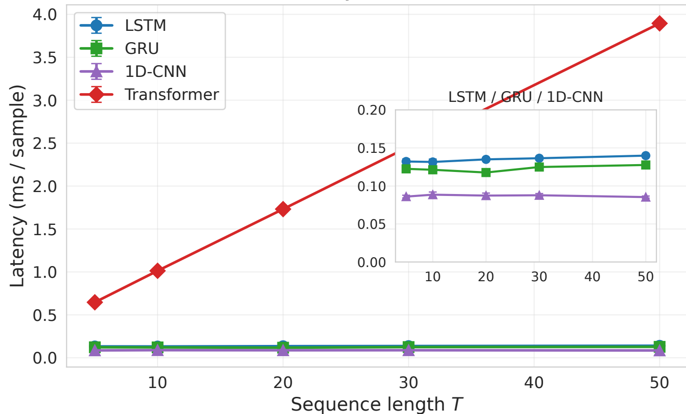
Inference latency vs T on NVIDIA A100
