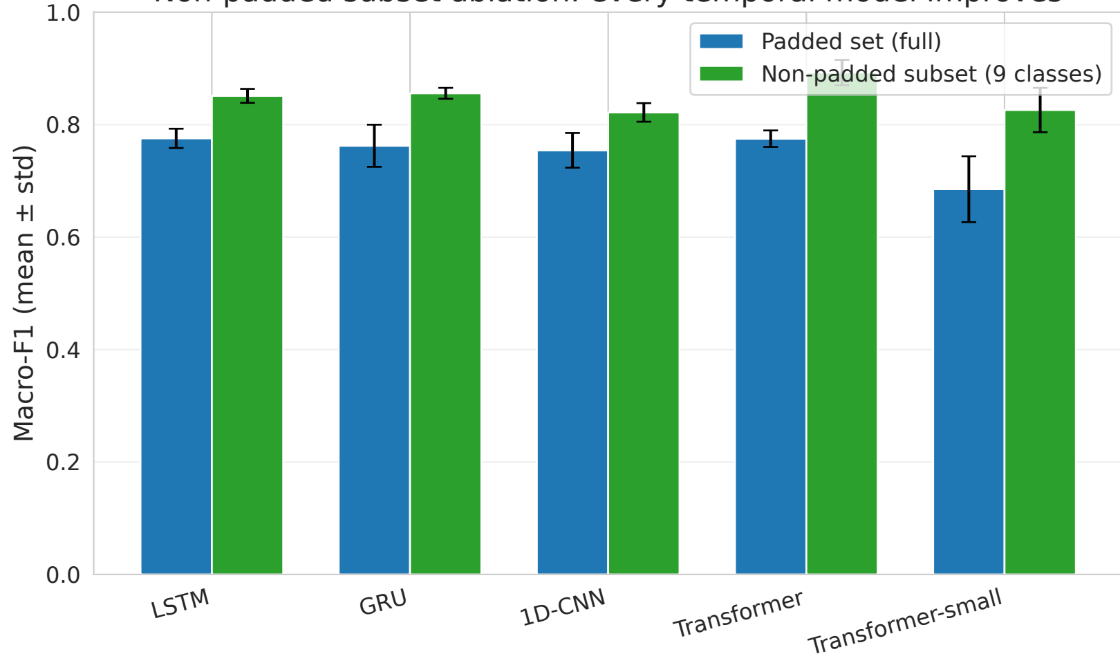
Non-padded subset ablation: every temporal model improves
