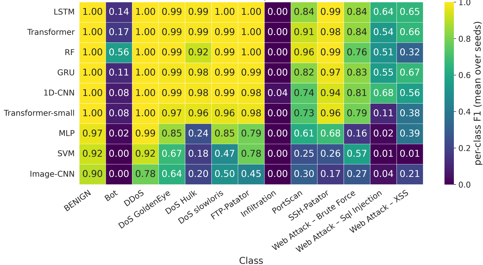
Per-class F1 (random 80/20 split, mean across seeds)
