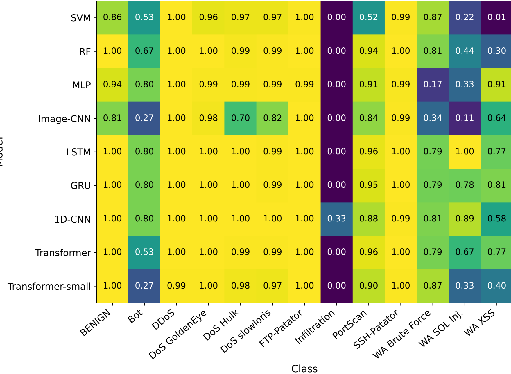
Per-class recall — random split (mean across seeds)
