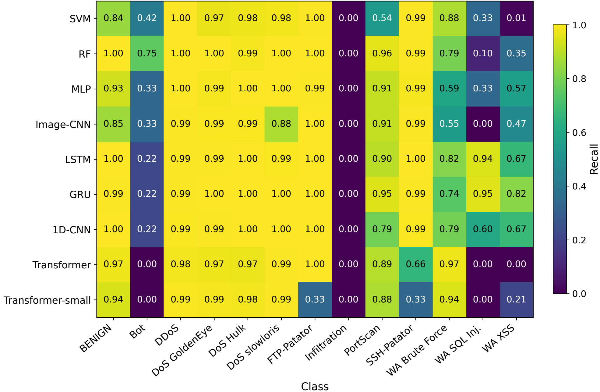
Per-class recall — group-by-5-tuple split (mean across seeds)
