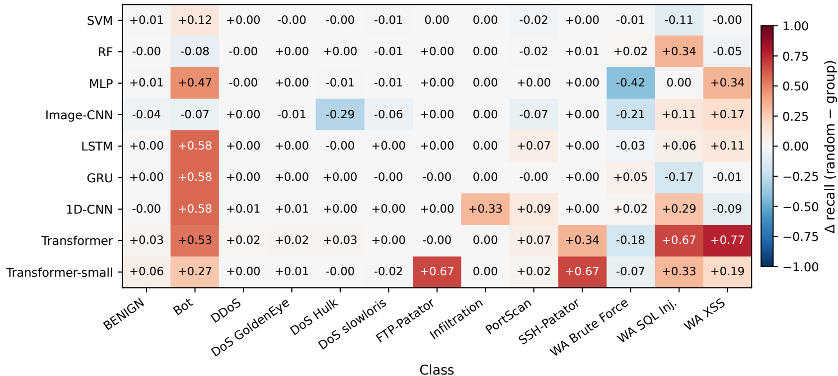
Per-class recall drop: random – group
