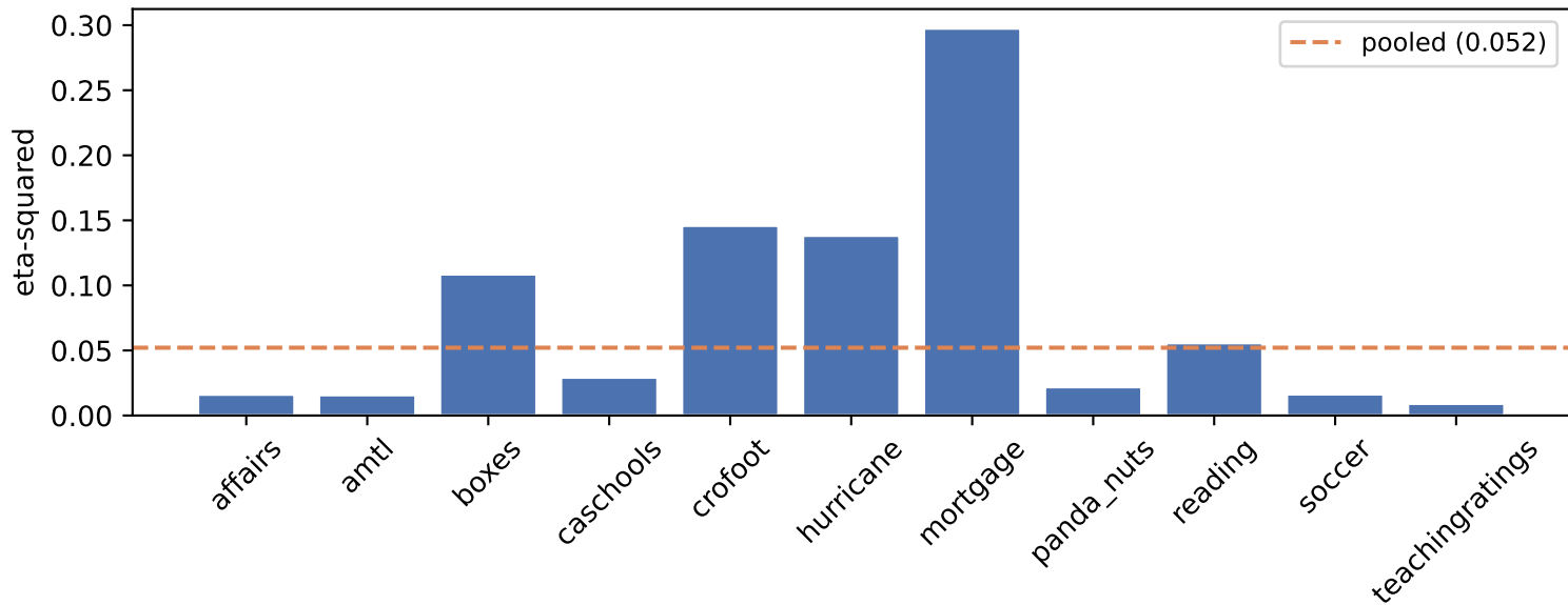
Variance in confidence scores explained by perturbation type
