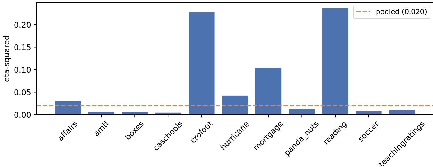
Variance in response scores explained by perturbation type
