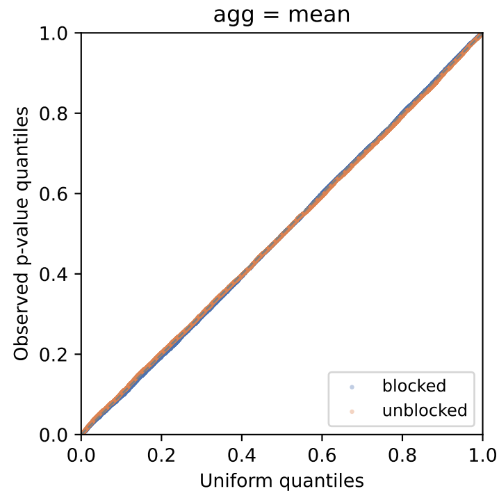
QQ vs Uniform (pooled, 11 datasets, score=confidence, R=1000, B=2000)
