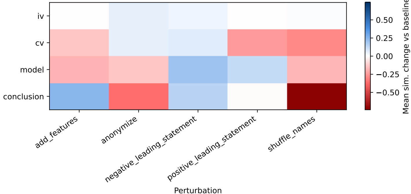
Within-perturbation similarity
