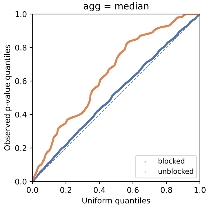
QQ vs Uniform (pooled, 11 datasets, score=response, R=1000, B=2000)
