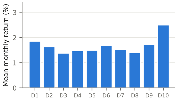
Volatility (60d)
