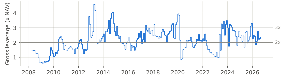
(b) V2 gross leverage at each rebalance
