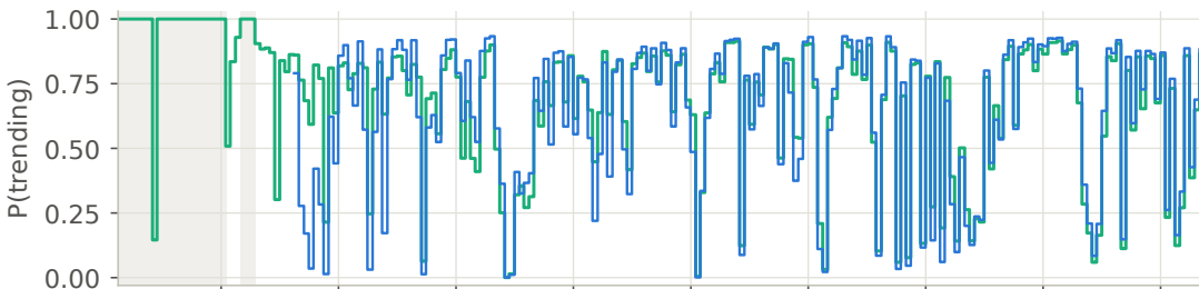
(b) R2: probability of the high-variance state of SPY (filtered)
