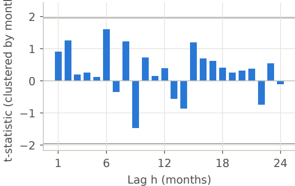
(a) Regressor: scaled return at lag h
