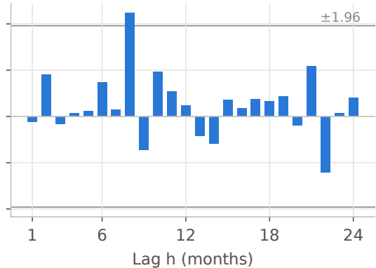
(b) Regressor: sign of return at lag h
