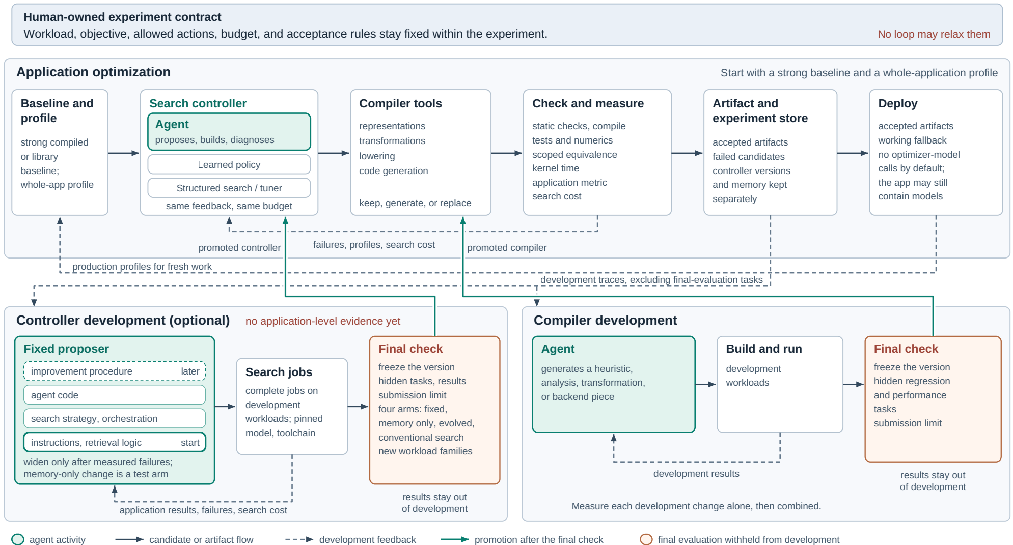
Figure 1. One possible starting architecture. Humans fix the experiment contract. In application optimization, an agent, a learned policy, and structured search propose candidates with the same feedback and budget; checks and measurement decide, and deployment needs no optimizer-model calls by default. Development traces exclude final-evaluation tasks. Compiler development and optional, late-stage controller development each iterate on development feedback, freeze a selected version for a hidden final check, and promote it only if it passes. Controller changes start with instructions or retrieval logic and widen only after measured failures. The three targets do not require three agents or permanent layers.
