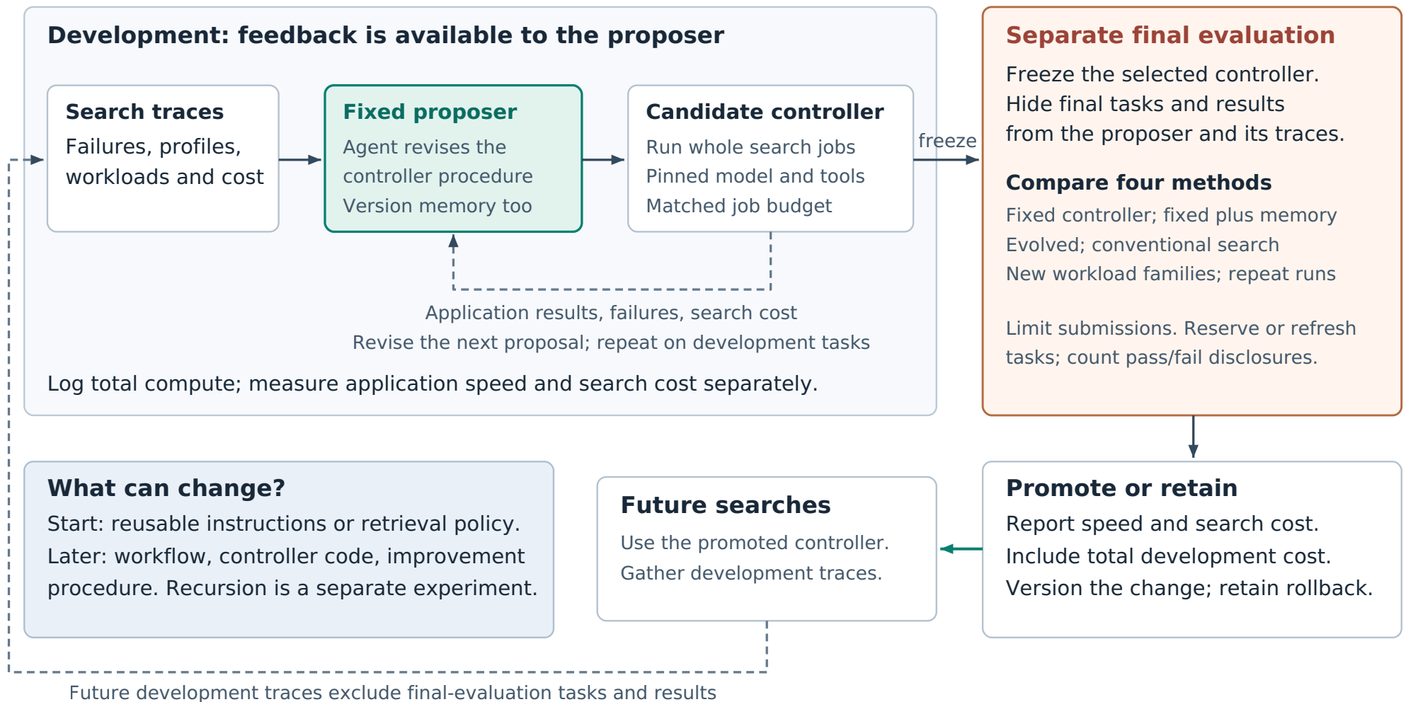
Figure 2. Controller development with a separate final evaluation. Development jobs return application results, failures, and search cost to the proposer. A selected controller is frozen before final evaluation; final tasks and results stay outside development feedback. Promotion affects future searches. Application-level benefit remains unproven in the reviewed evidence; recursive improvement is a further experiment.
