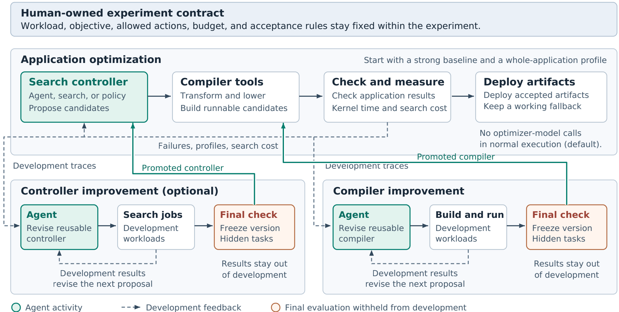
Figure 1. One possible starting architecture. Each development loop uses application-search evidence and returns development results to its proposer. Selected versions face separate final evaluation before promotion. The three targets do not require three agents or permanent layers. Normal execution reuses accepted artifacts; online optimizer calls remain an optional design choice.
