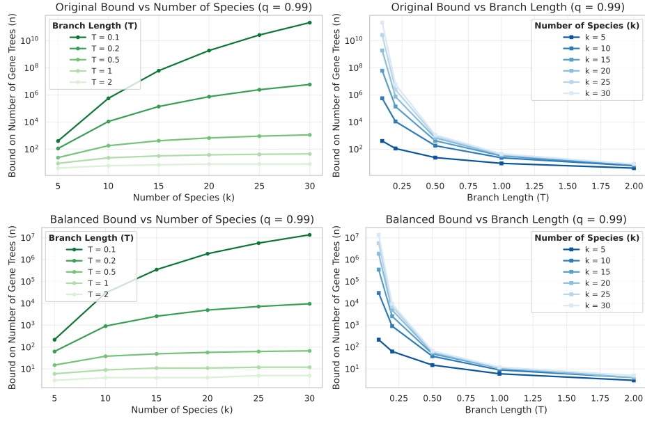
Figure 2.5: Bipartition cover bounds as functions of the two key parameters: k , T_{\min} . (top) The original bound [81]. (bottom) Our balanced bound (Theorem 2.2.9)
