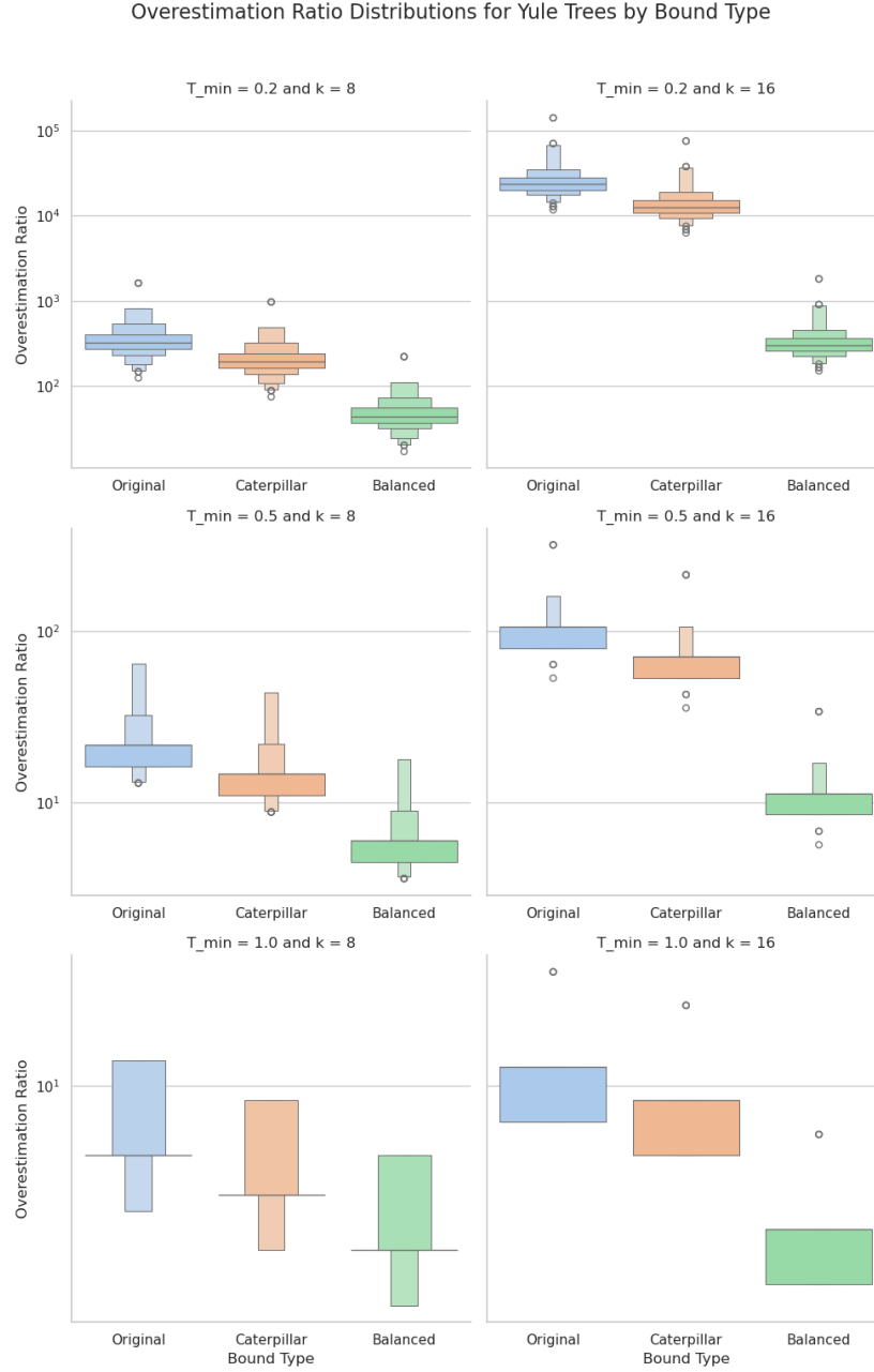
Figure 2.9: Log-scaled overestimation ratios for Yule trees. Rows vary T_{\min} \in \{0.2, 0.5, 1\} and columns vary k \in \{8, 16\} ; nested boxes show progressively wider quantile intervals around the median (25–75%, 12.5–87.5%, 6.25–93.75%, and 3.125–96.875%).
