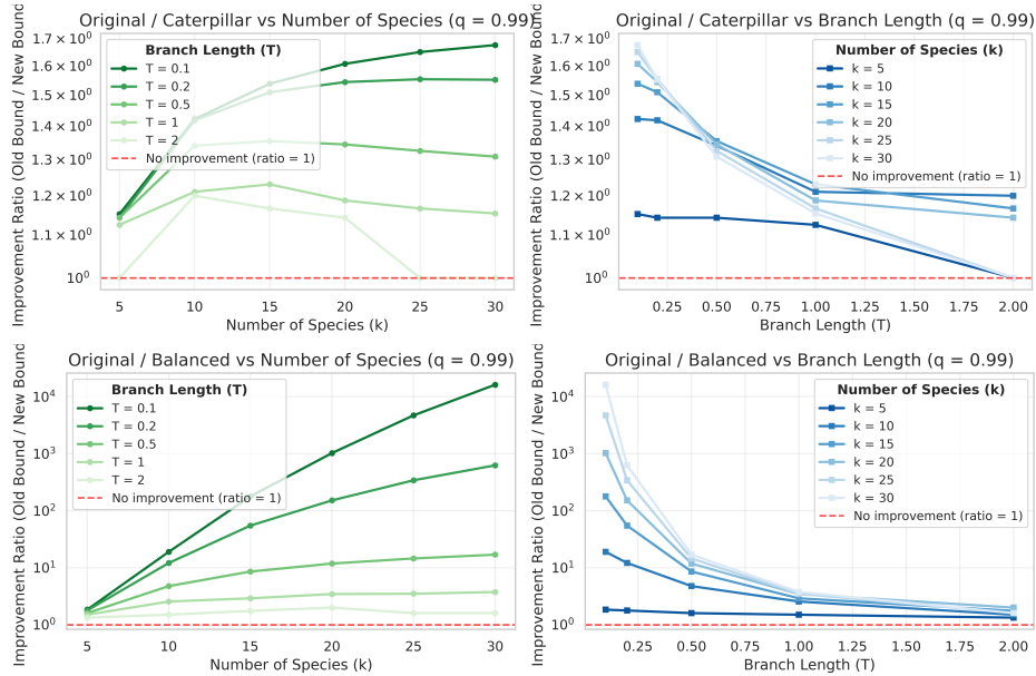
Figure 2.6: Improvement ratios. (top) Improvement of caterpillar bound (Theorem 2.2.3) over the original bound (Theorem 2.1.1). (bottom) Improvement of the balanced bound over original
