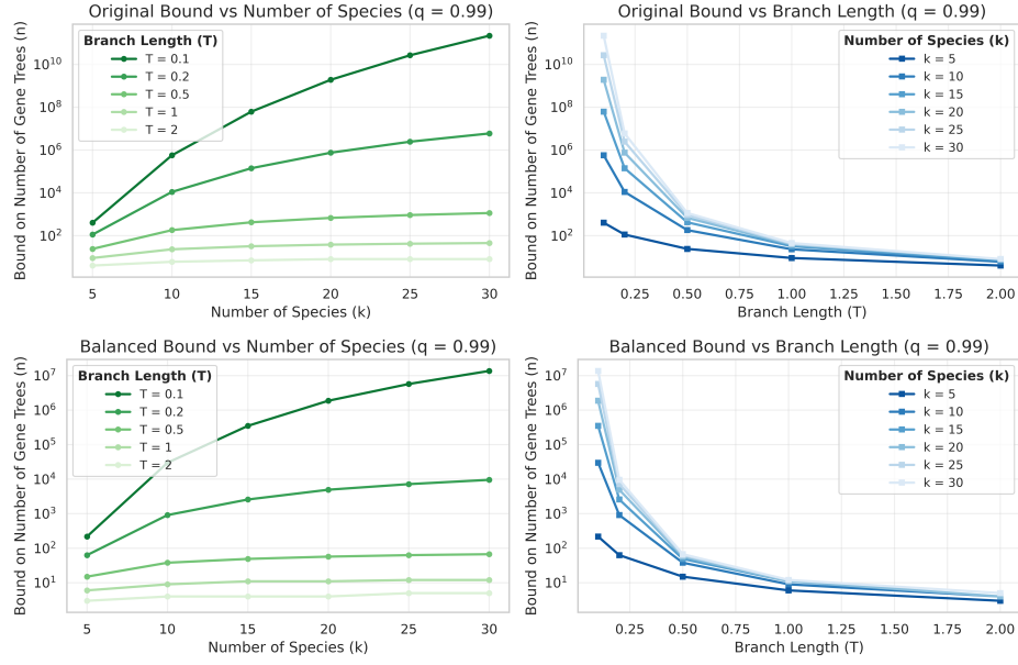
Figure 1.5: Bipartition cover bounds as functions of the two key parameters: k , T_{\min} . (top) The original bound [80]. (bottom) Our balanced bound (Theorem 1.2.9)
