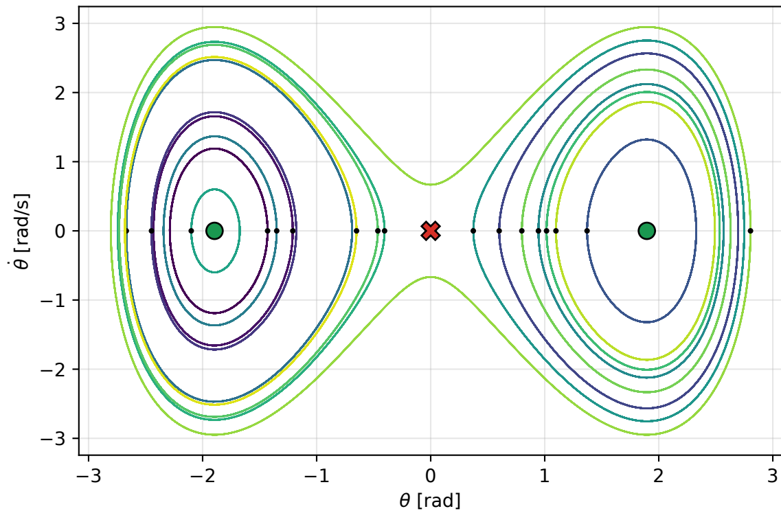
Phase plane, k = 0.5 k_{cr} (20 runs, t \in [0, 60] s)
