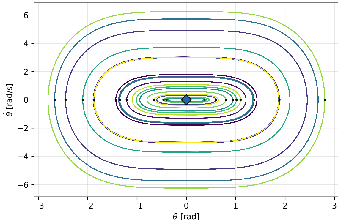
Phase plane, k = k_{cr} (20 runs, t \in [0, 60] s)
