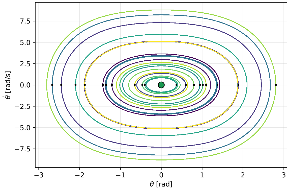
Phase plane, k = 1.5 k_{cr} (20 runs, t \in [0, 60] s)
