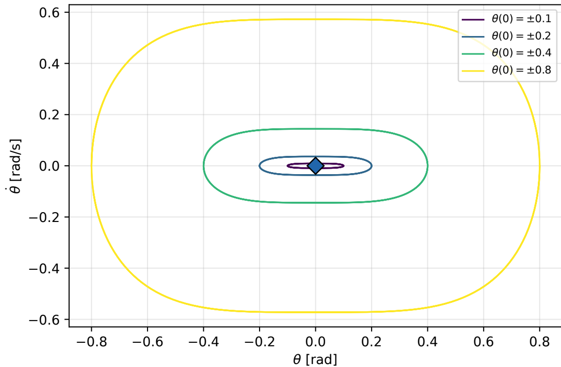
Zoom near upright equilibrium, k = k_{cr}
