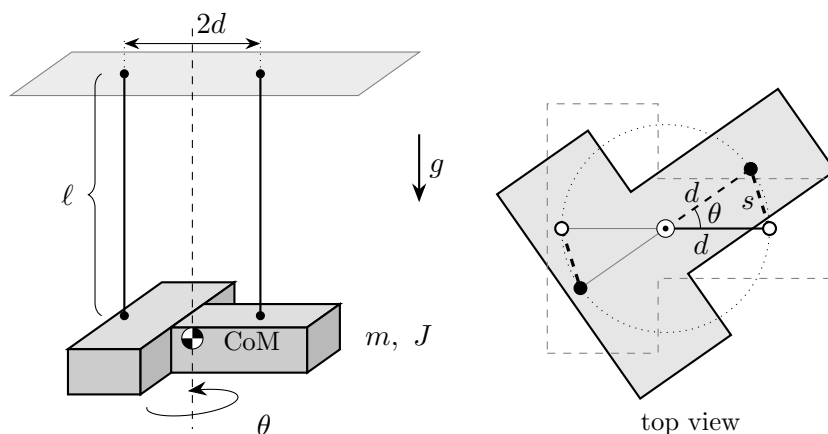
Figure 2: The T-shaped body from Problem 1 hung as a bifilar pendulum. Left: oblique view at rest; the strings attach to the top of the body on its x axis, a distance d on either side of the CoM. Right: top view with the body twisted by \theta about the vertical axis through its center of mass (pointing out of the page). Open circles mark where the strings attach to the ceiling (fixed); filled circles mark where they attach to the body. The thick dashed segments of length s are the horizontal projections of the strings. Drawings are not to scale.
