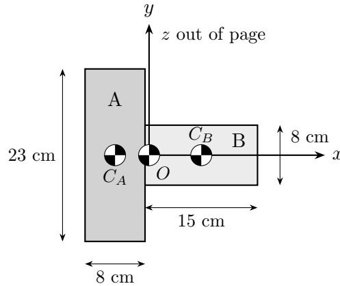
Figure 1: Top view of the T-shaped body, made of box A (the crossbar) and box B (the stem). Both boxes are 5 cm thick in the z direction, with their mid-planes at z = 0 . The body-frame origin O is at the center of mass of the T-shaped body, and C_A and C_B mark the centers of mass of the two boxes.
