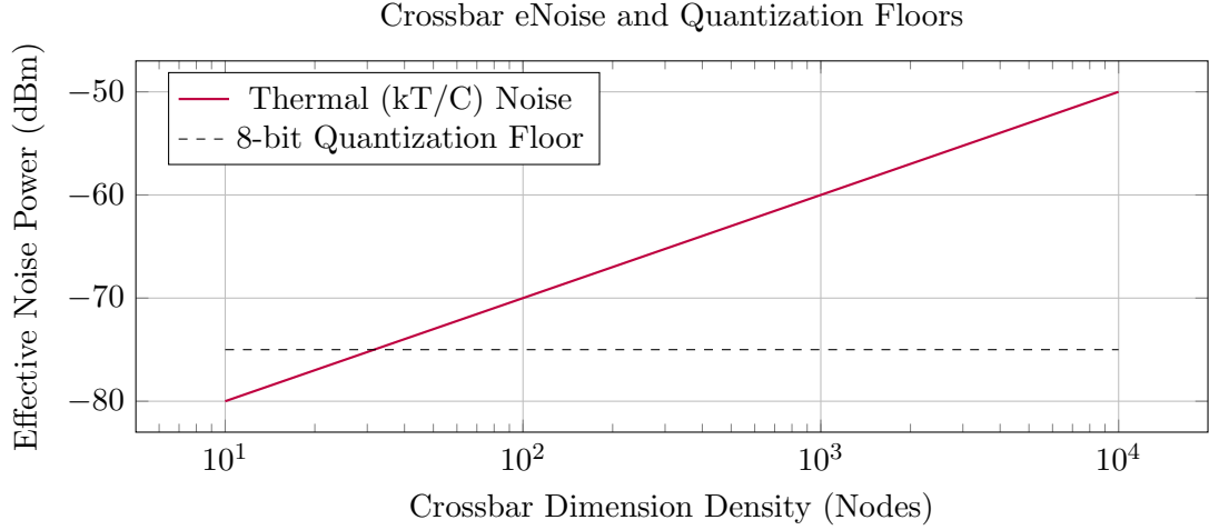
Figure 9.3: Crossbar eNoise Profile. Spectral analysis of quantization boundaries and thermal kT/C drift at the structural crossbar level. ( Analytical Profile ) — Theoretical curve computed from the closed-form bound. Empirical simulation data for this measurement is available at the companion portal (§9.5).
