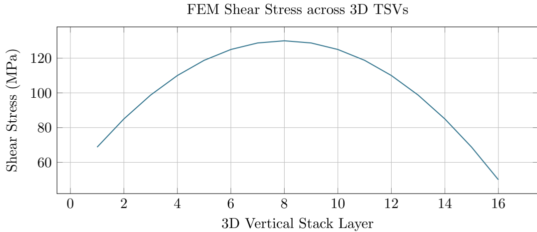
Figure 9.12: Shear Stress FEM Analysis. Multi-physics simulation of mechanical strain on the dense 3D vertical Through-Silicon Vias (TSVs), showing peak stress accumulation at the middle interconnect layers.
