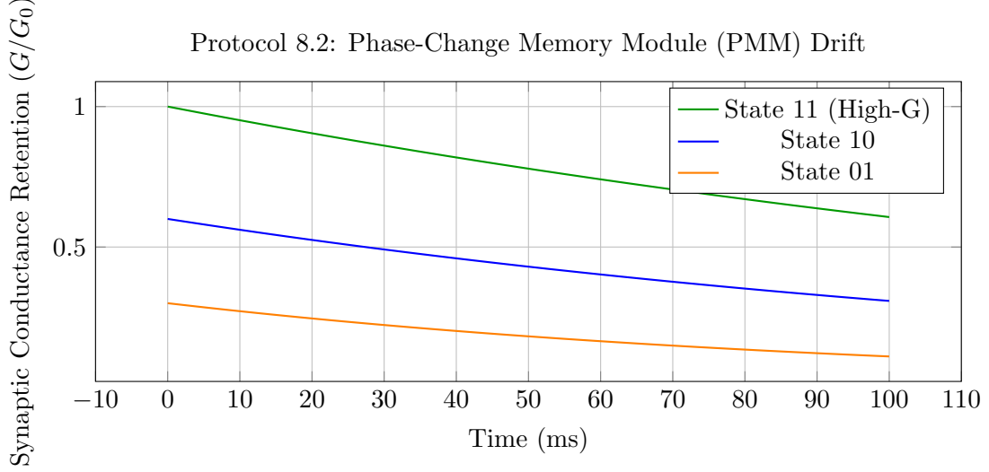
Figure 9.5: Protocol 8.2: PMM Retention. Demonstrates convergence and retention probabilities across layered synaptic densities, highlighting structural relaxation drift in chalcogenide glass. ( Simulation Result ) — Extracted from simulation executed on the APU-X layout model. Full simulation artefacts available at the companion portal (§9.5).
