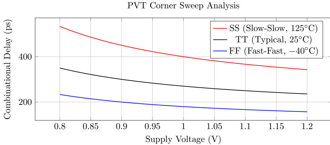
Figure 9.8: Process, Voltage, and Temperature (PVT) Corner Sweep. SPICE empirical analysis of worst-case and best-case propagation delays across corner extremes.
