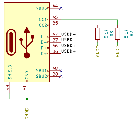
J1 USB_C_Receptacle_USB2.0_16P
