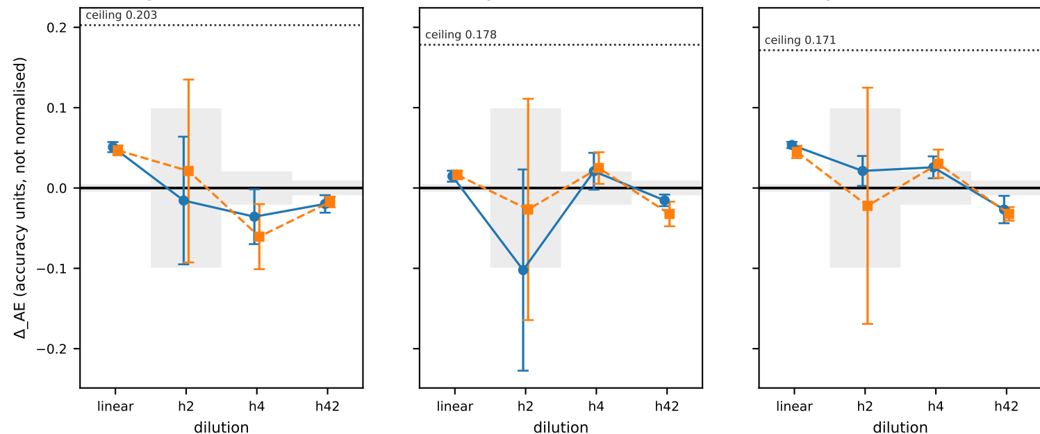
1b. \Delta_{\text{AE}} along the dilution axis, per generator seed, 95 % CI
