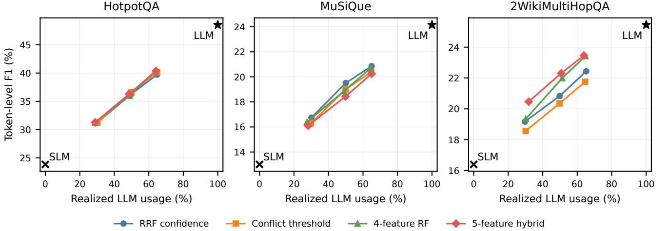
Fig. 1. F1 against realized LLM usage. Crosses and stars denote Always-SLM and Always-LLM; connected points correspond to 30%, 50%, and 65% target budgets.
