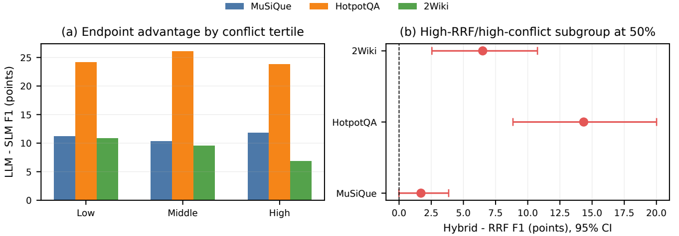
Fig. 2. Exploratory failure-mode analysis. (a) High conflict does not imply a monotonically larger LLM advantage. (b) Nevertheless, at the 50% target the hybrid recovers errors missed by RRF inside the label-free high-RRF/high-conflict subgroup on HotpotQA and 2Wiki.
