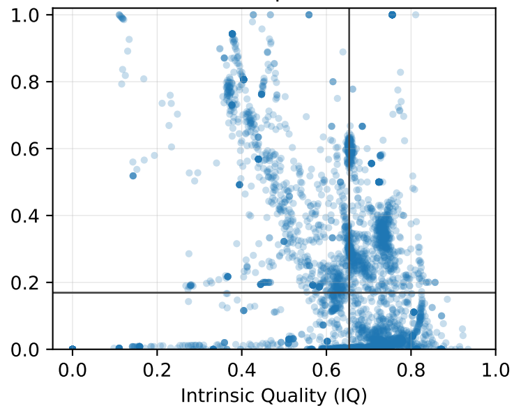
DeepFD
