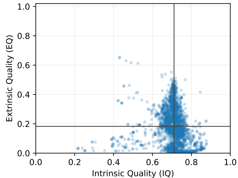
CleanML
