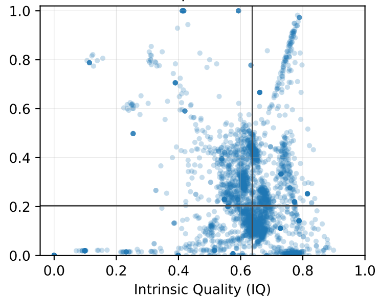
DeepLocalize
