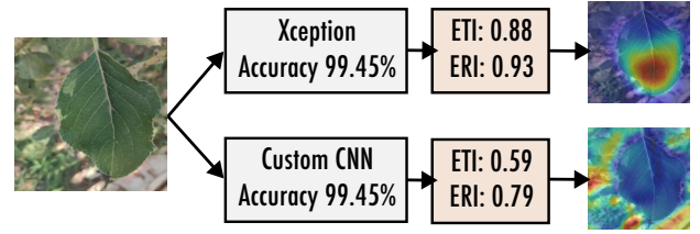
Figure 1: Comparison between traditional accuracy and the proposed XAI-based metrics (ETI and ERI). Although both Xception and the custom CNN achieve identical 99.45% validation accuracy, Grad-CAM heatmaps reveal that the custom CNN relies on background context. The proposed ETI and ERI metrics successfully capture this flaw by producing lower scores for the custom model.
