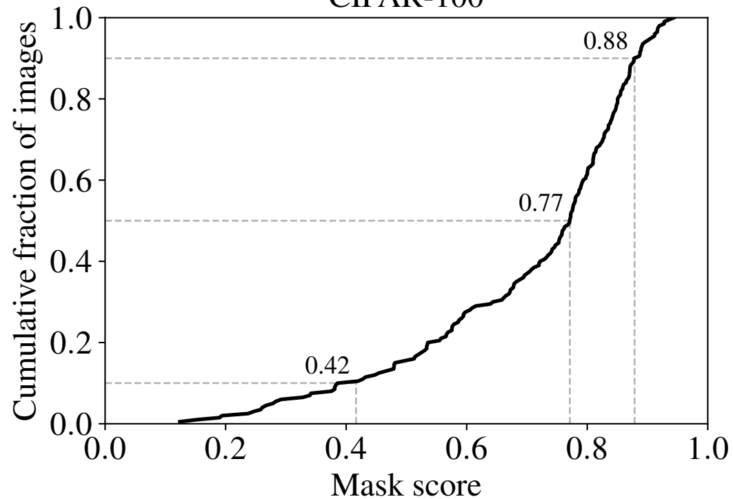
CIFAR-100
